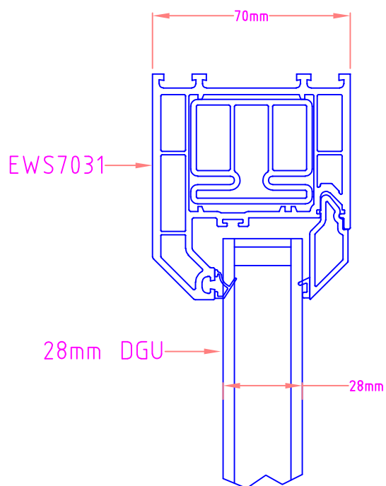
Section through Fan Light
