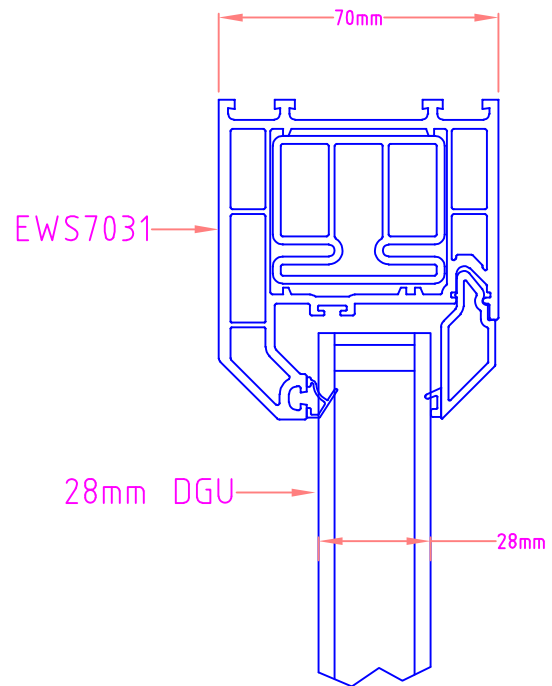
Section through Side Light
