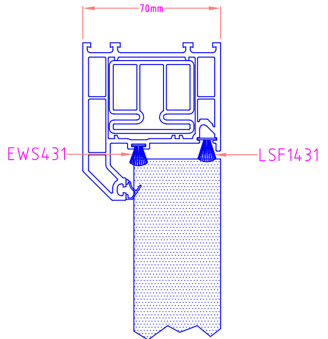
Section through Side Light
