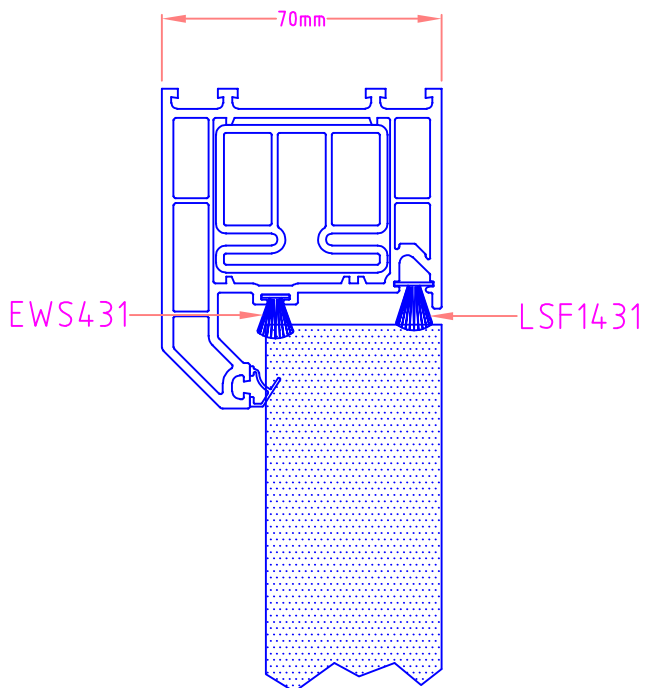
Section through Door
