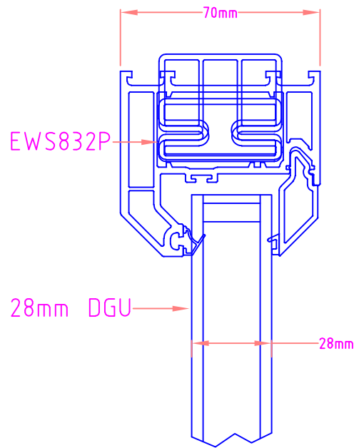
Section through Side Light
