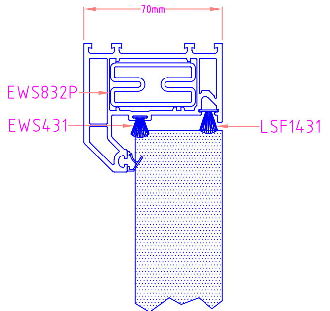
Section through Side Light
