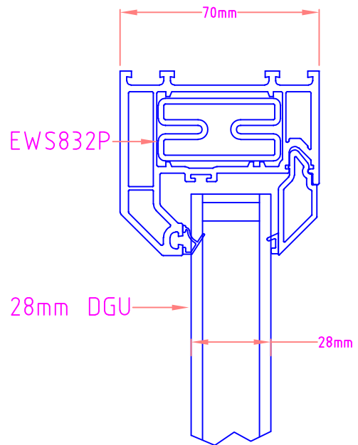
Section through Side Light
