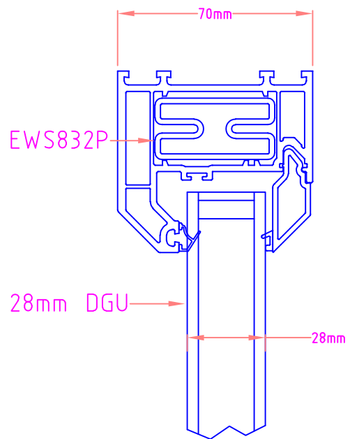
Section through Fan Light
